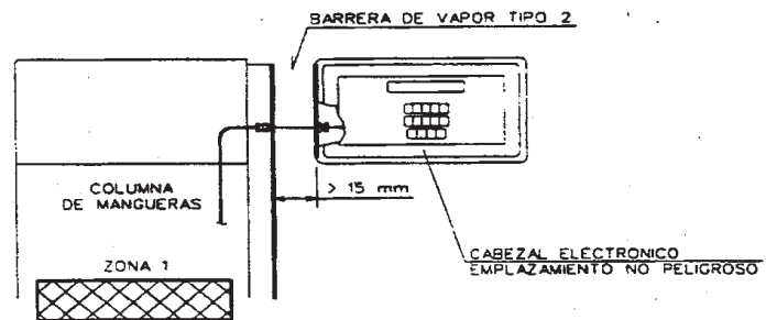
DETALLE "E"
